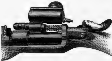
SNIDER BREECH-ACTION RIFLE.
